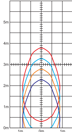
Abstand Leuchte Wand (LW) = 1,0m
